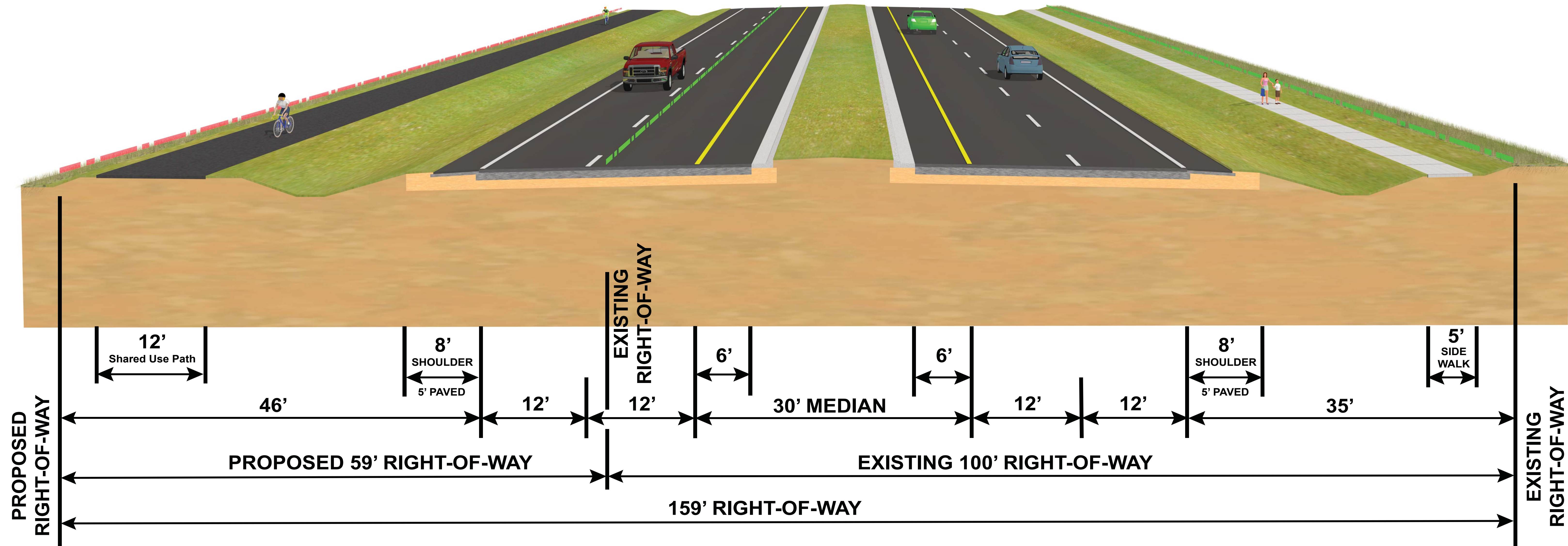
Typical Section 3A Suburban Roadway
