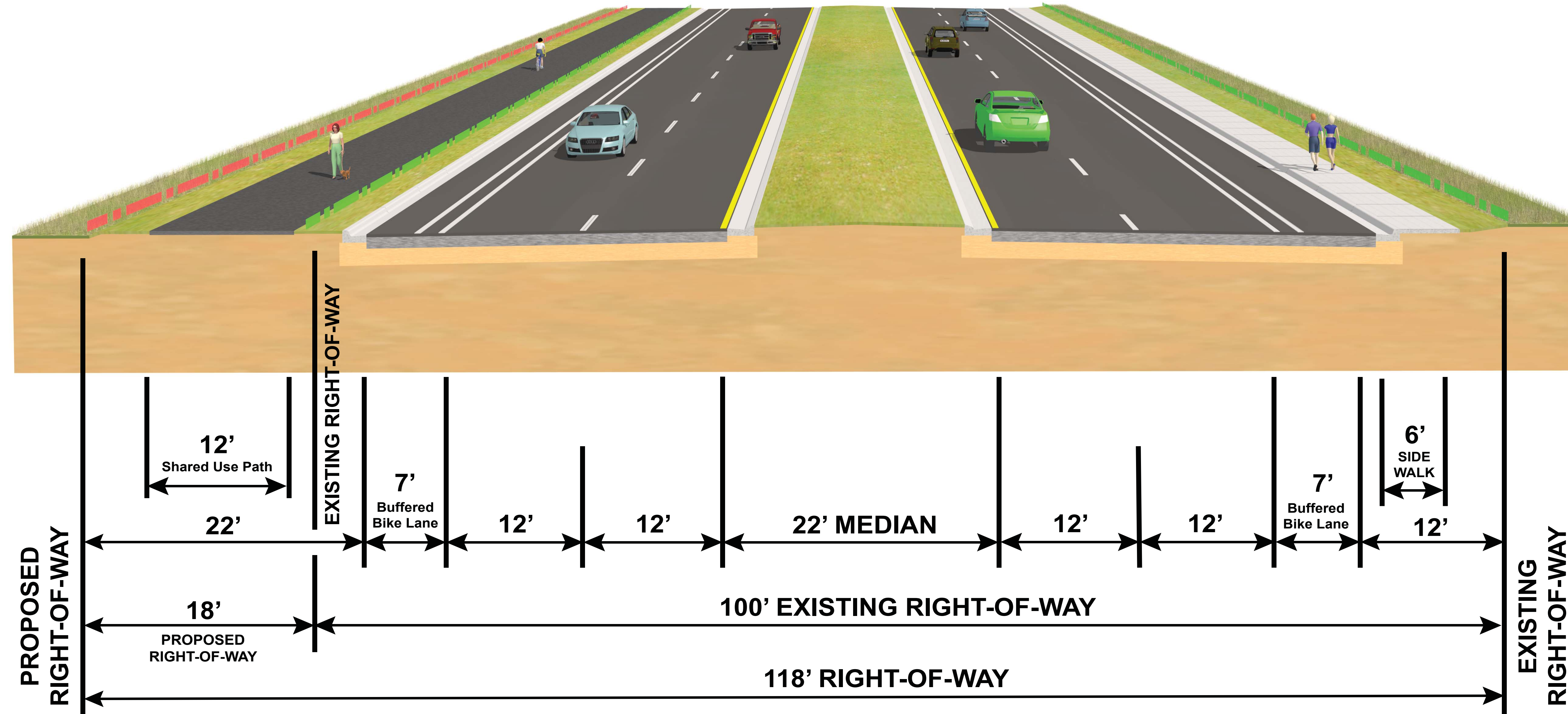
Typical Section 1B Urban Roadway
