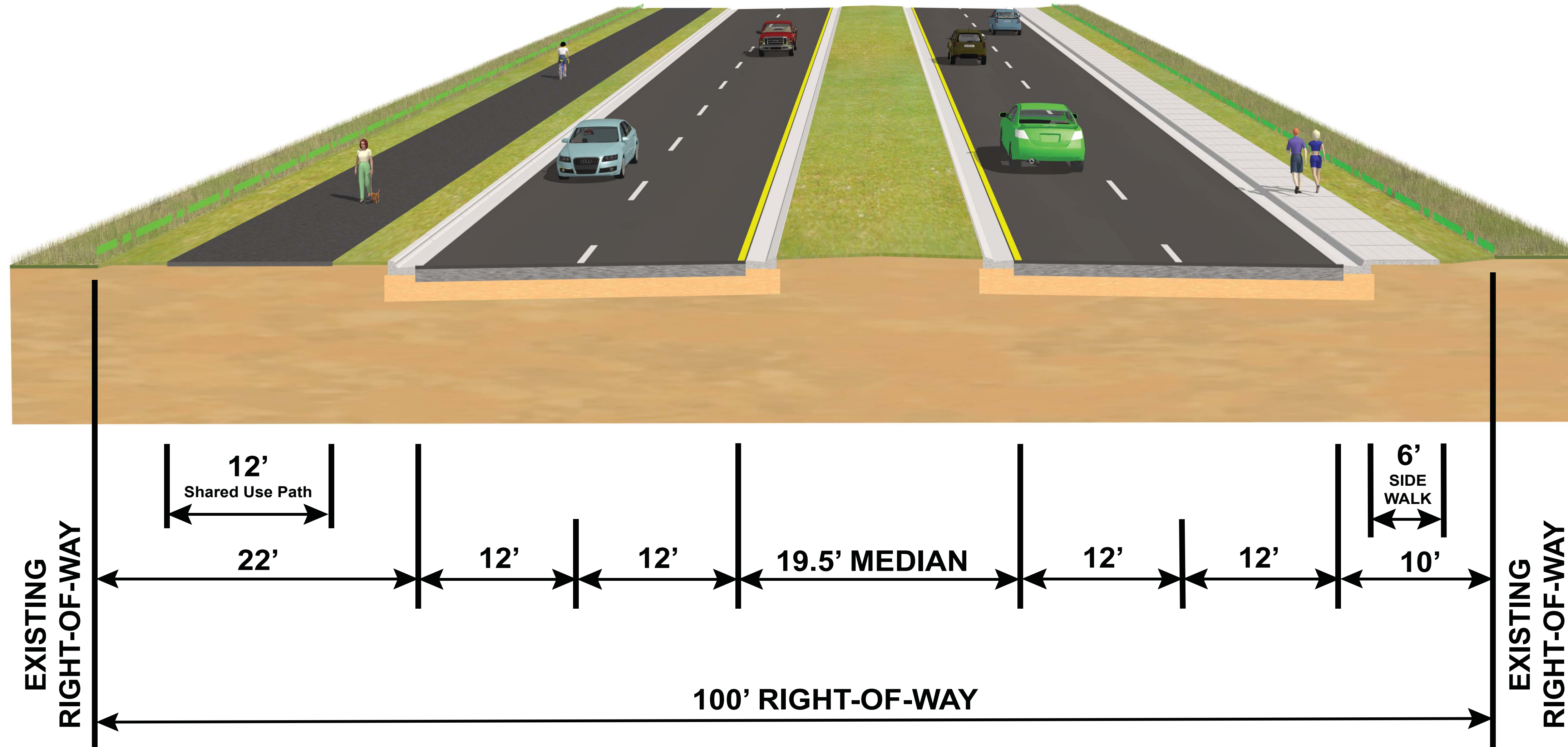
Typical Section 1A Urban Roadway
